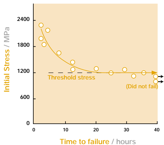
Figure 6. The effect of initial stress on time to failure of maraging steel in 3.5% NaCl solution.
