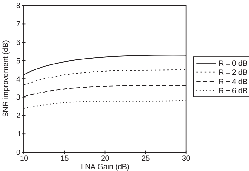
Figure 9.5 SNR improvement as a function of LNA gain and rise. The graph is generated using the following assumptions: L_1 = 2.0 dB, F_2 = F'_4 = 6.0 dB, F'_2 = 2.2 dB, L'_1 = 0.5 dB, L'_3 = 1.5 dB.
