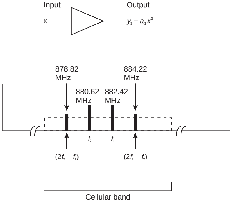
Figure 9.10 Third-order IM components in the cellular band. Note that a_2=1 , A=1 , and B=1 .
