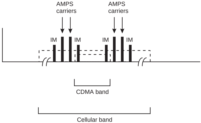
Figure 9.11 Third-order IM components are generated by adjacent AMPS carriers and fall within the CDMA band.
